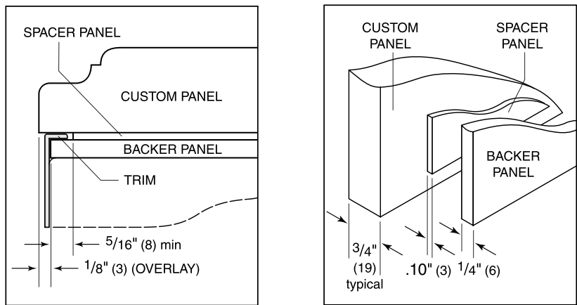
Panel assembly (cross section).
