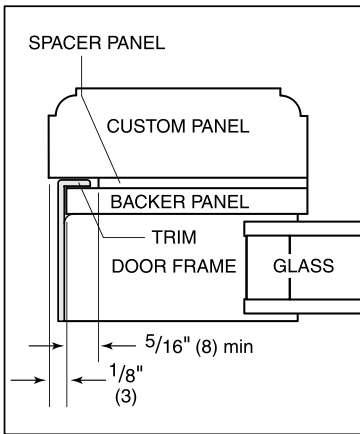
Panel assembly (cross section).
